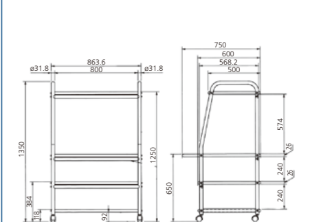
PC rack (for all models)
