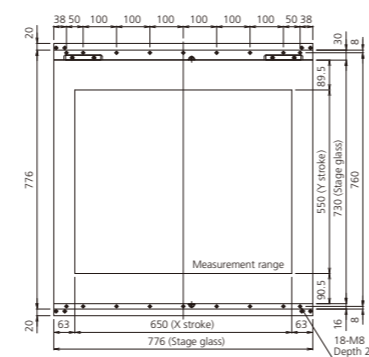
Top view of stage
