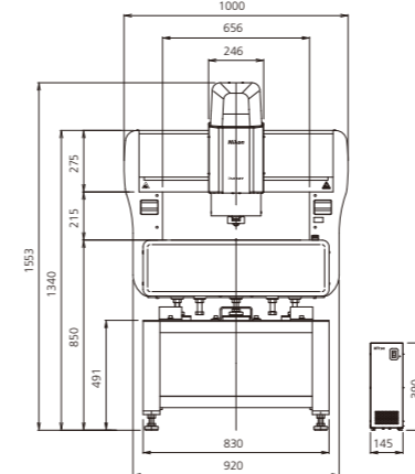
Dimensional diagram
