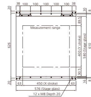
Top view of stage
